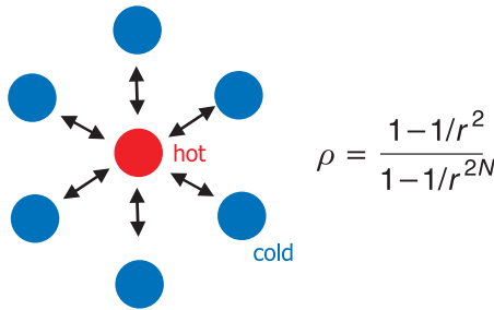
Figure 8.10 It is possible to find graphs that amplify selection over drift. The “star” is a good example. For large N , a mutant with relative fitness r has a fixation probability \rho = (1 - 1/r^2)/(1 - 1/r^{2N}) . Therefore a relative fitness r on a star is equivalent to a relative fitness r^2 in the Moran process. The star is an amplifier of selection.
